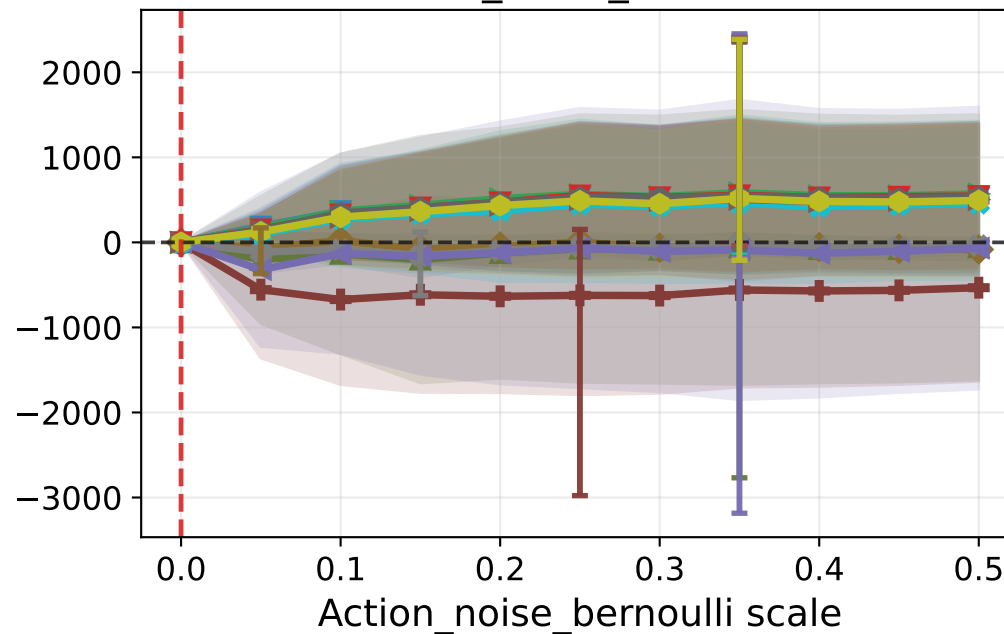
Action_noise_bernoulli
