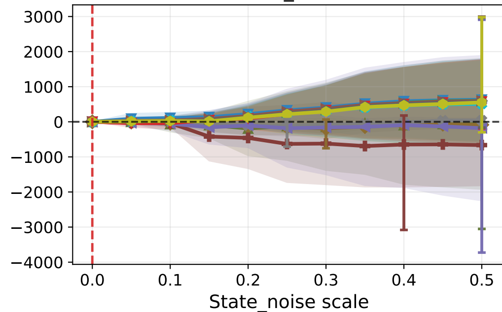
State_noise
